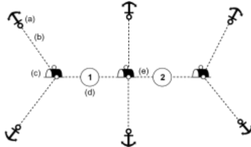
Figure 8-2 – Mooring trot
