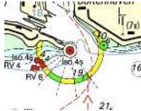
Paper Chart Symbol
