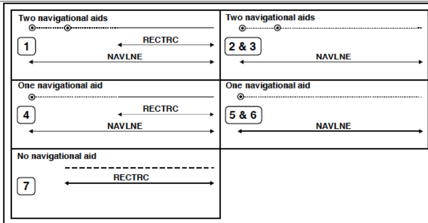
Figure 15-5 – Navigation lines – Geometry encoding
