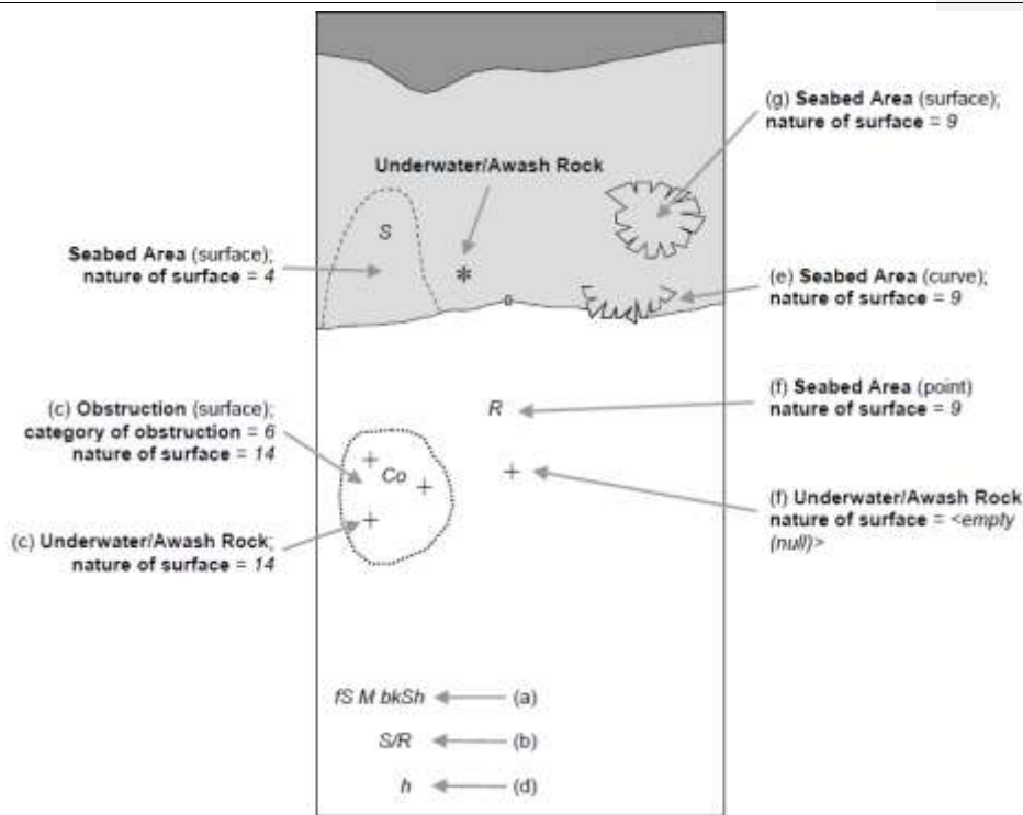
Figure 12-1 – Seabed areas
