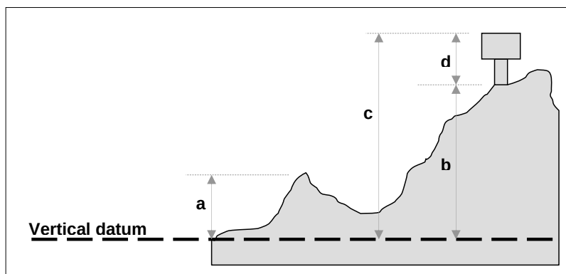
Figure 2-2 – Heights and elevations
