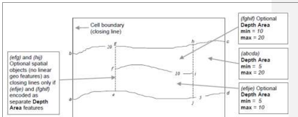
Figure 11-3 – Geometry of depth areas
