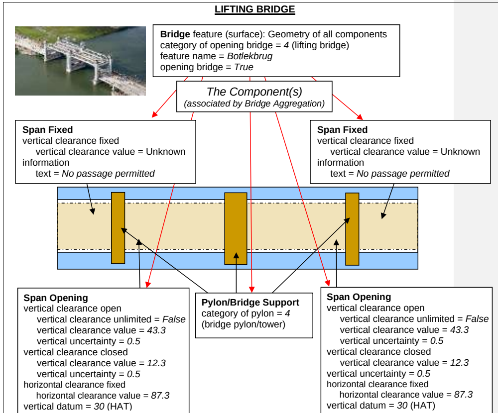
Figure 6-6 – Lifting bridge – Example
