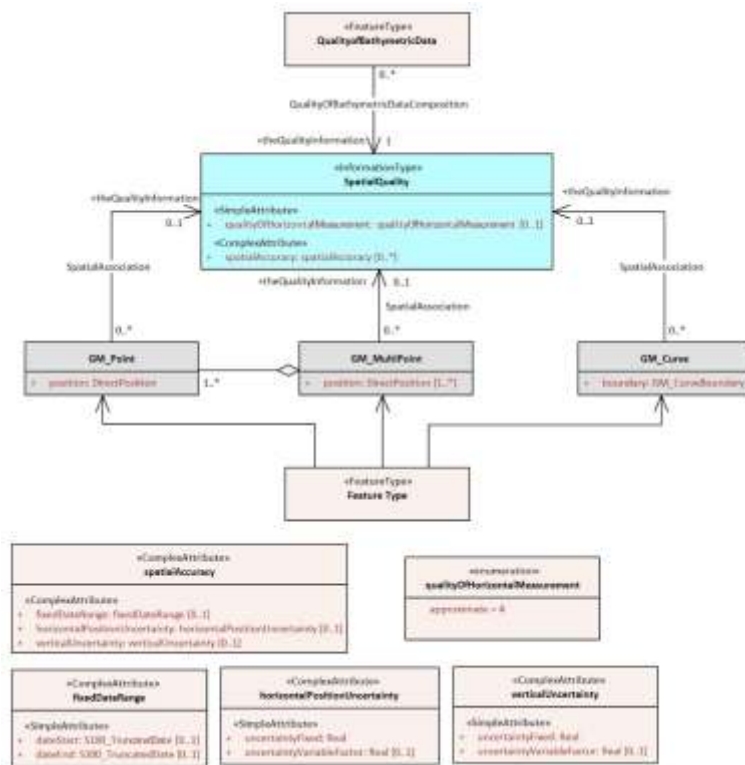
Figure 2-1 – Spatial Quality information type
