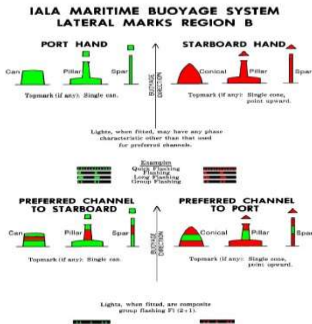
Figure 20-1 – IALA lateral buoys – Characteristics
