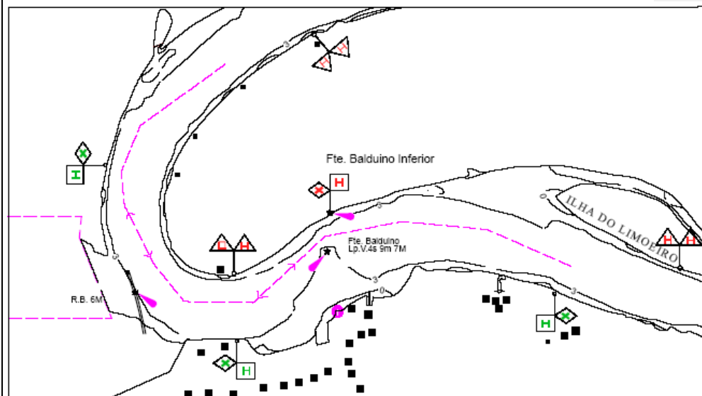
Diagram for Paraguay-Parana waterway - Brazilian complementary aids
