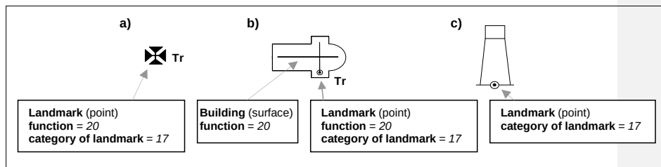
Figure 6-1 – Landmarks
