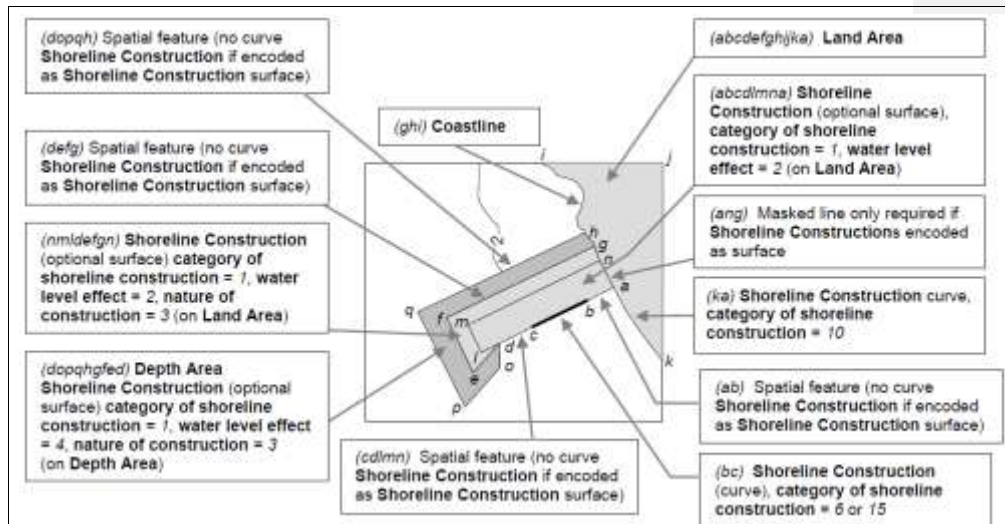
Figure 8-1 – Shoreline constructions
