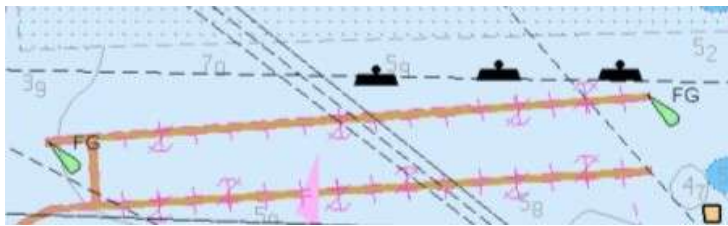
Figure 2-5 – Overwriting symbols – Example
