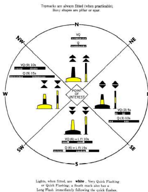
Figure 20-6 – IALA cardinal beacons – Characteristics
