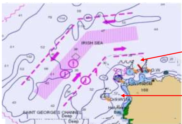
Figure 2-9 – Traffic Separation Scheme with appropriate masking
